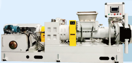
SILICONE STRAINING MACHINE 200 / 250
