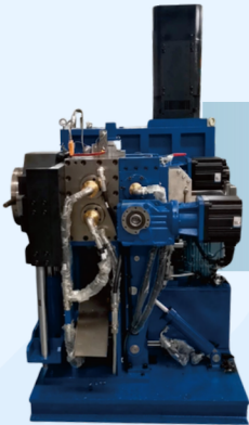
HOT FEEDING GEAR PUMP STRAINER MACHINE GS-1000 / GS-1500 / GS-2000 / GS-3000 / GS-5000
